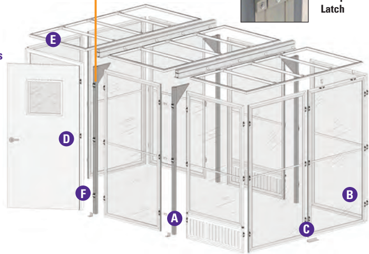
MODEL 250 1"x 2" Tubing for taller rooms
